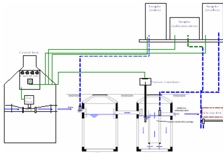
Figure 1. Technical infiltration system from KME-Mall with monitoring devices.
