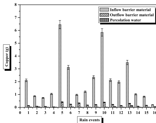
Figure 4. Performance of the retention facility I regarding copper elimination.
