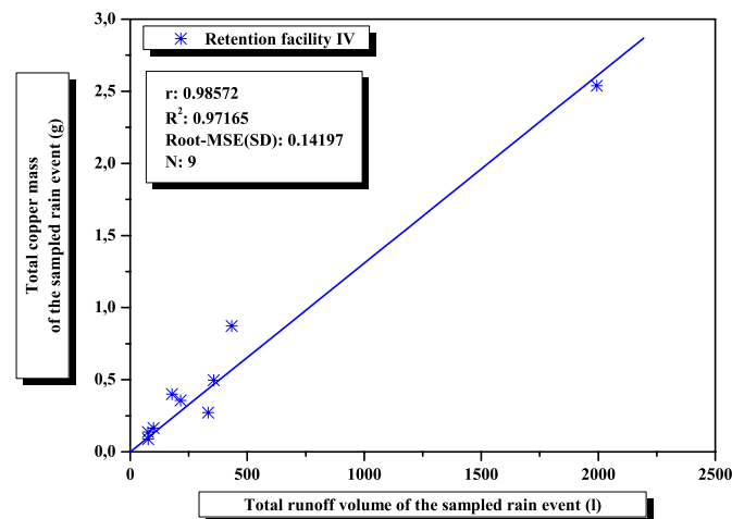
Figure 3. Linear correlation between the copper mass washed off the roof surface during a rain event and the runoff volume of the rain event, in spring.
