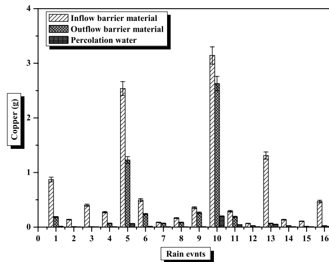
Figure 5. Performance of the retention facility IV regarding copper elimination.
