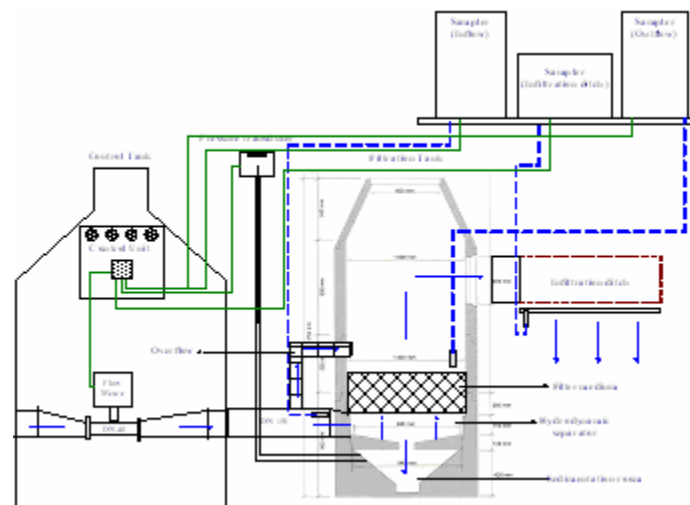
Figure 2. Technical infiltration system from HydroCon with monitoring devices.
